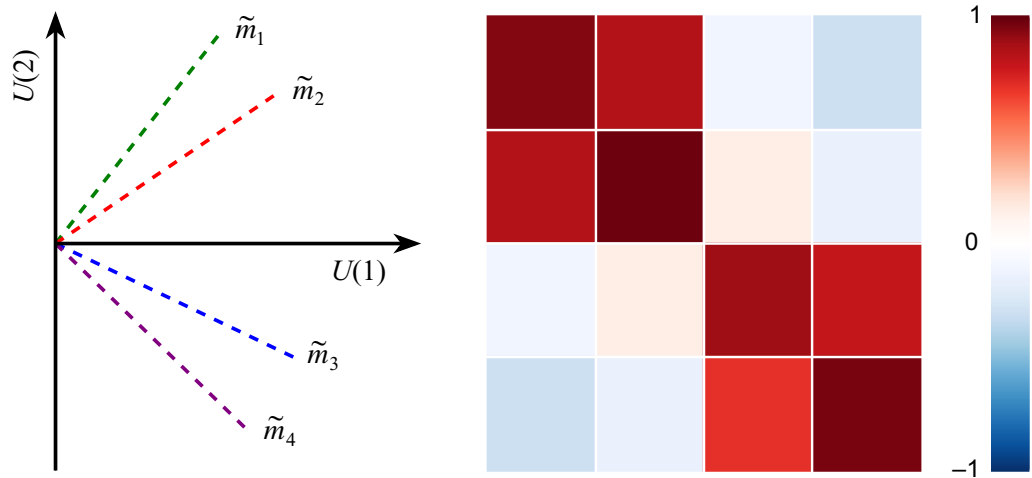
Figure 3. Schematic plot of the interrelation between the modular projections of four modules. The matrix represents the overlap computed as the scalar product between directions.
