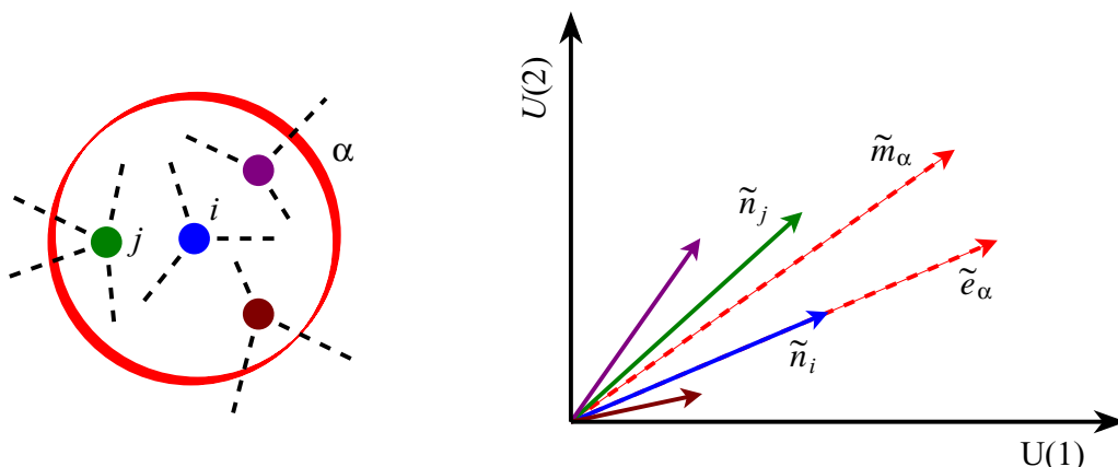
Figure 1. Geometrical scheme of the TSVD. The intramodular projection of module \alpha , \tilde{e}_\alpha is the direction where all internal nodes lie (in the plot, node i ). The node contribution projections \tilde{n} are represented by vectors in different colors. Finally, the modular projection \tilde{m}_\alpha is computed as the vector sum of all the node contribution projections belonging to it. Note that the intramodular projection and the modular projection do not coincide; the differences between both inform about the cohesiveness of the module.
