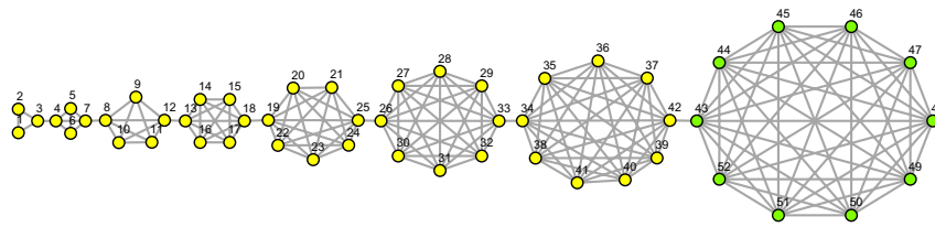
(b) Cliques line partition 8 modules
