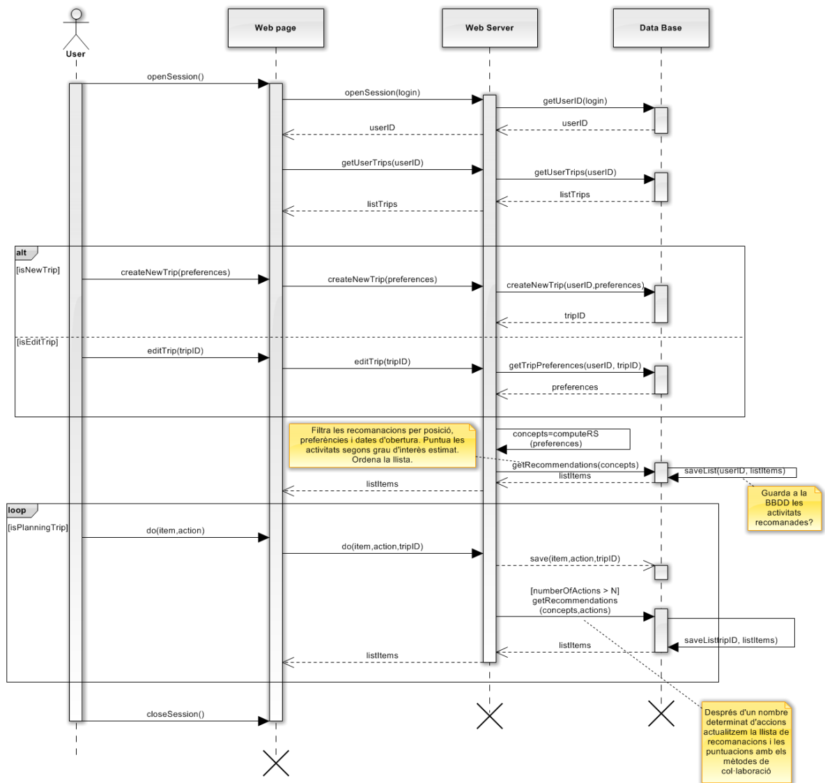
Figure 32. Sequence diagram
