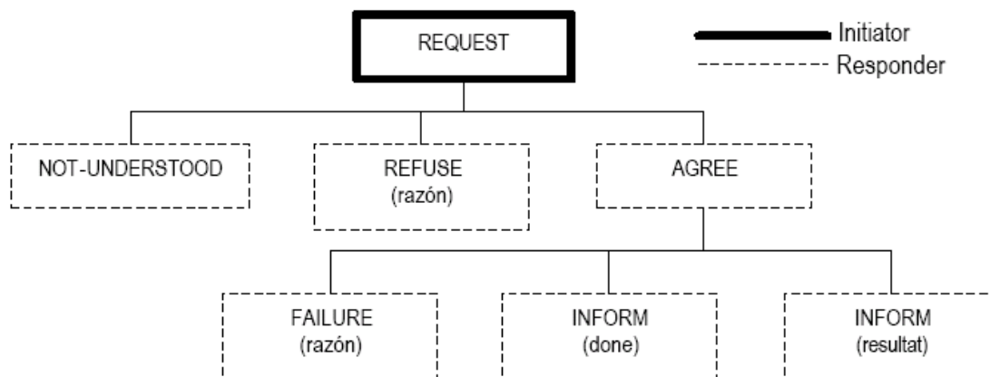
Protocolo FIPA-Request
